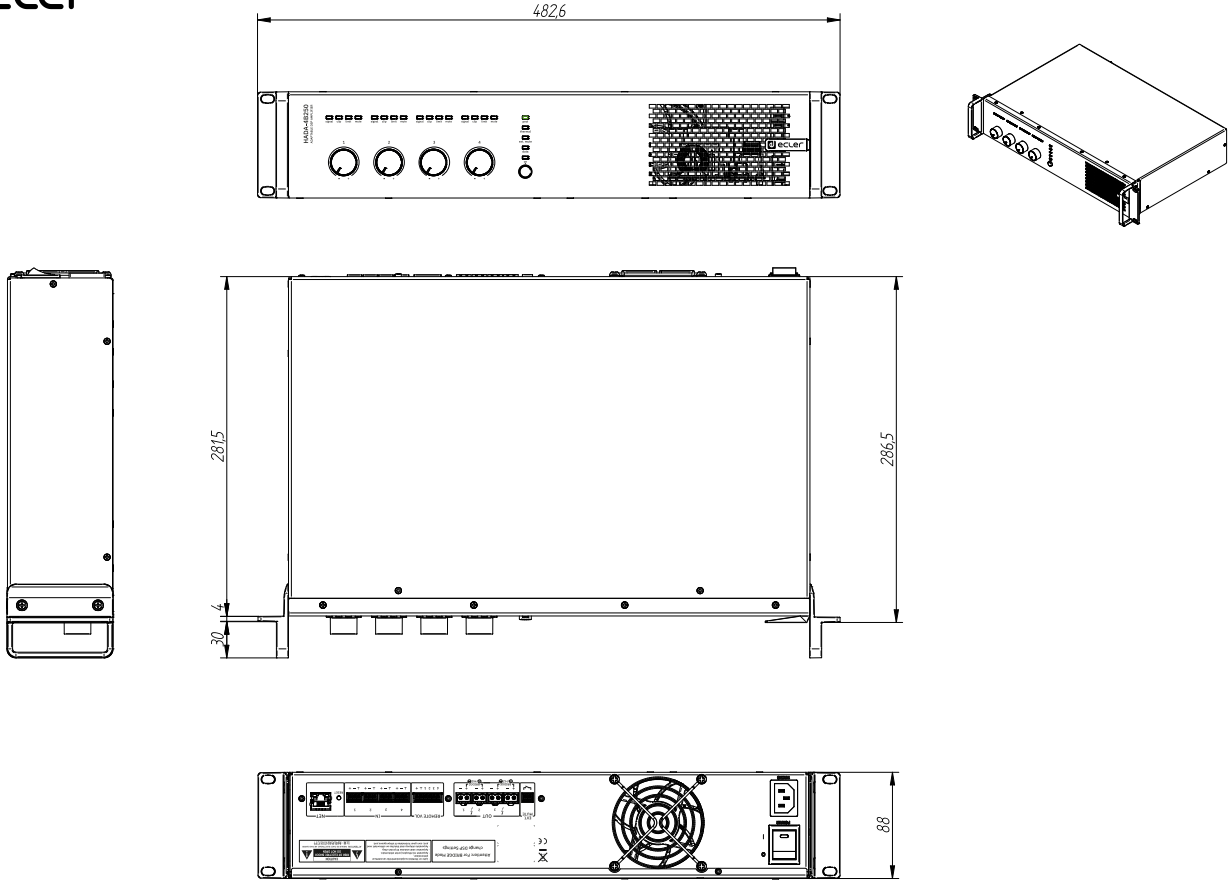
Ecler HADA-4B250 Mechanical Diagram
