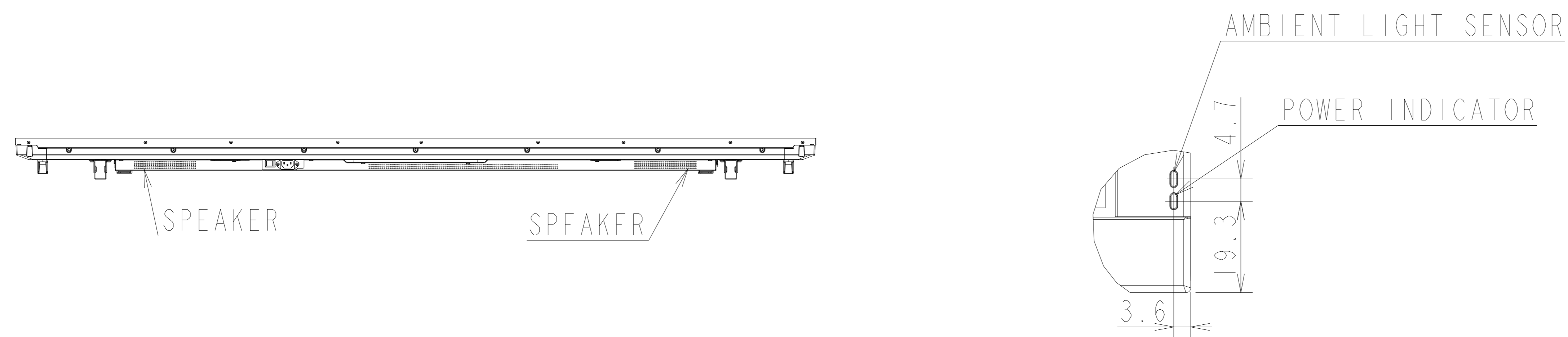
DETAIL A
